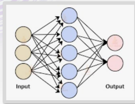
Neural Network
